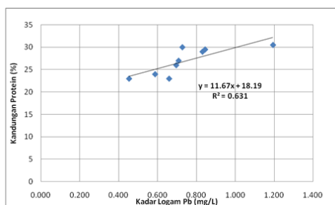
Gambar 4. Korelasi kadar logam Pb dan kandungan protein
